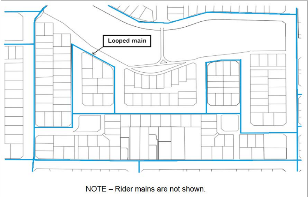
Figure 6.7 – Looped principal mains
