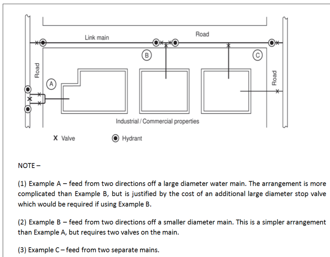
Figure 6.4 – Secure connection
