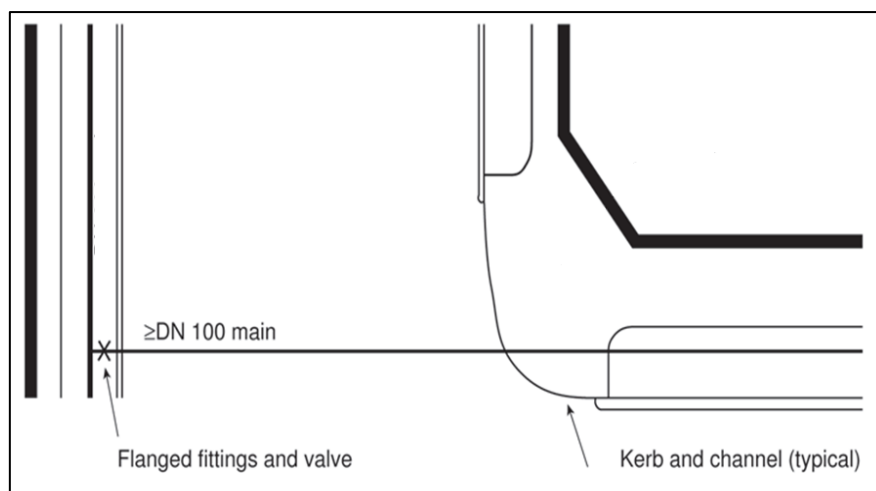
Figure 6.2 – Branch valve adjacent to main
