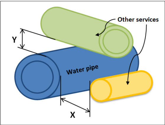
Figure 6.1 Service clearance measurements
