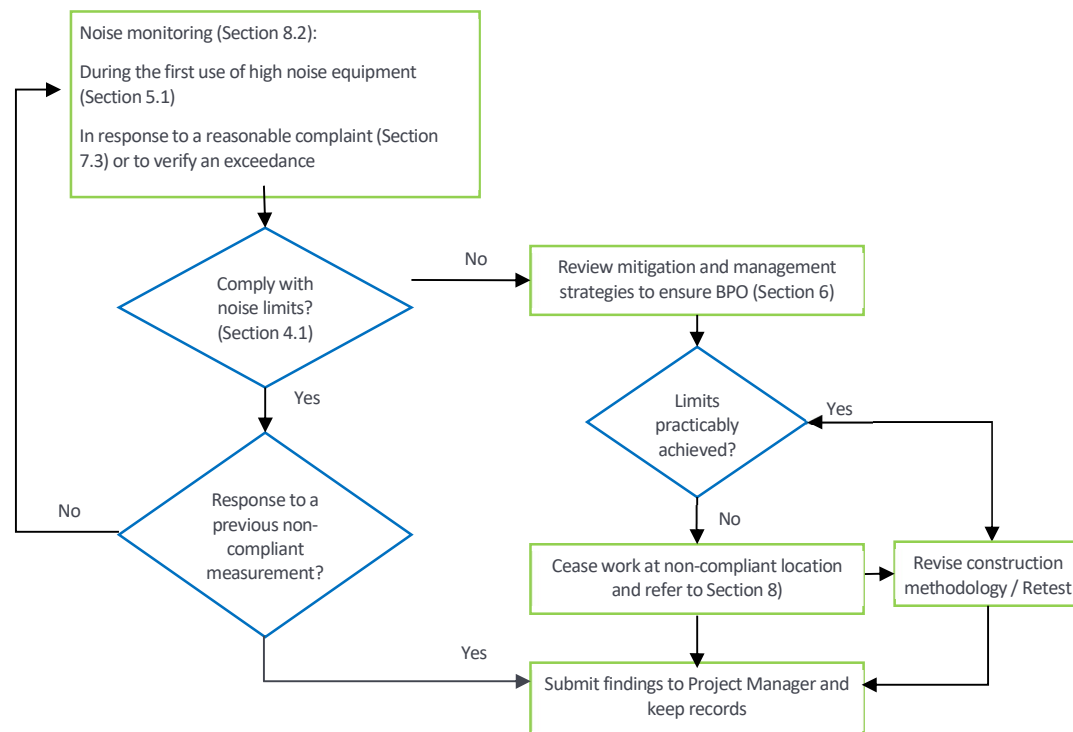
Figure 6: Noise Monitoring Flow Chart
