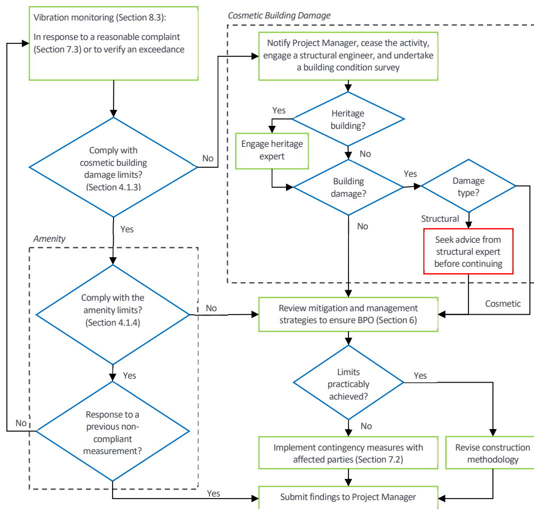
Figure 7: Vibration Monitoring Flow Chart
