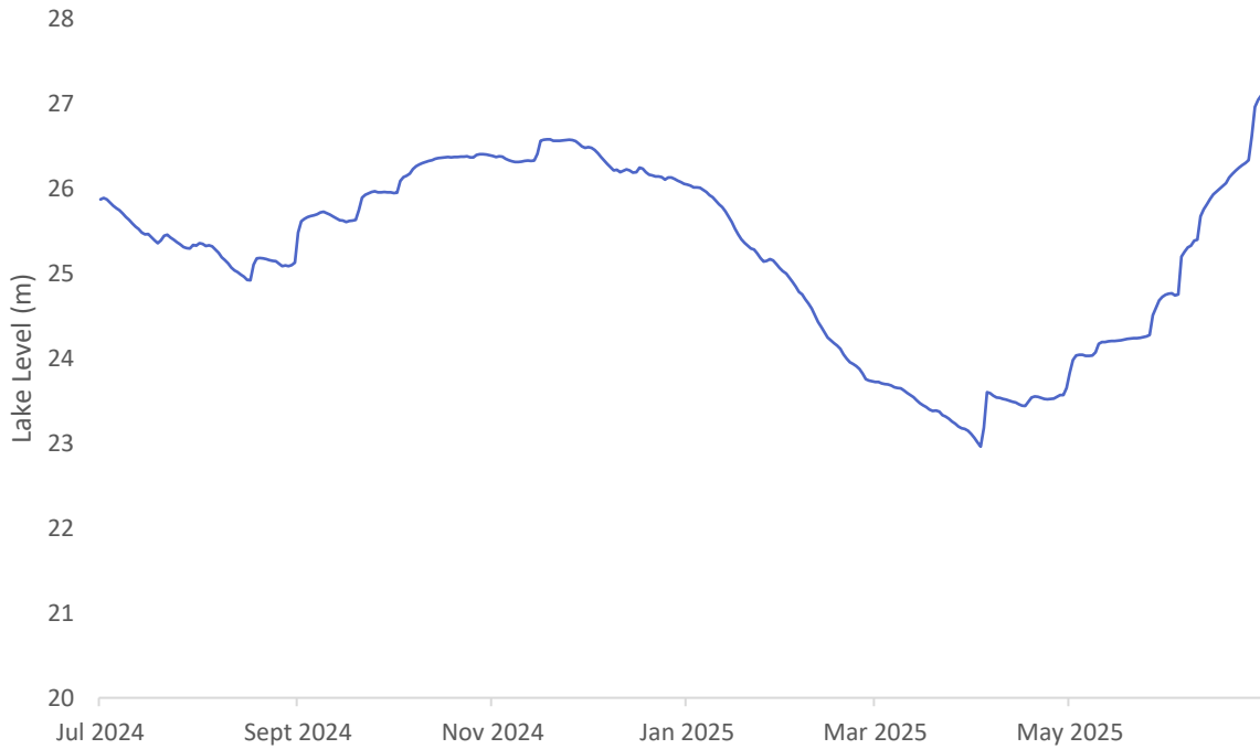
Figure 3-1: Reservoir daily average level for Cosseys Dam for the reporting period 2024-2025.
