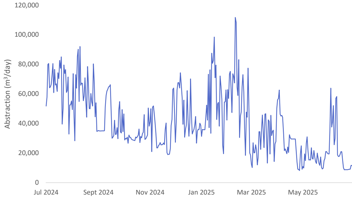
Figure 2-1: Total daily abstraction from Cosseys Dam for the reporting period 2024-2025.
