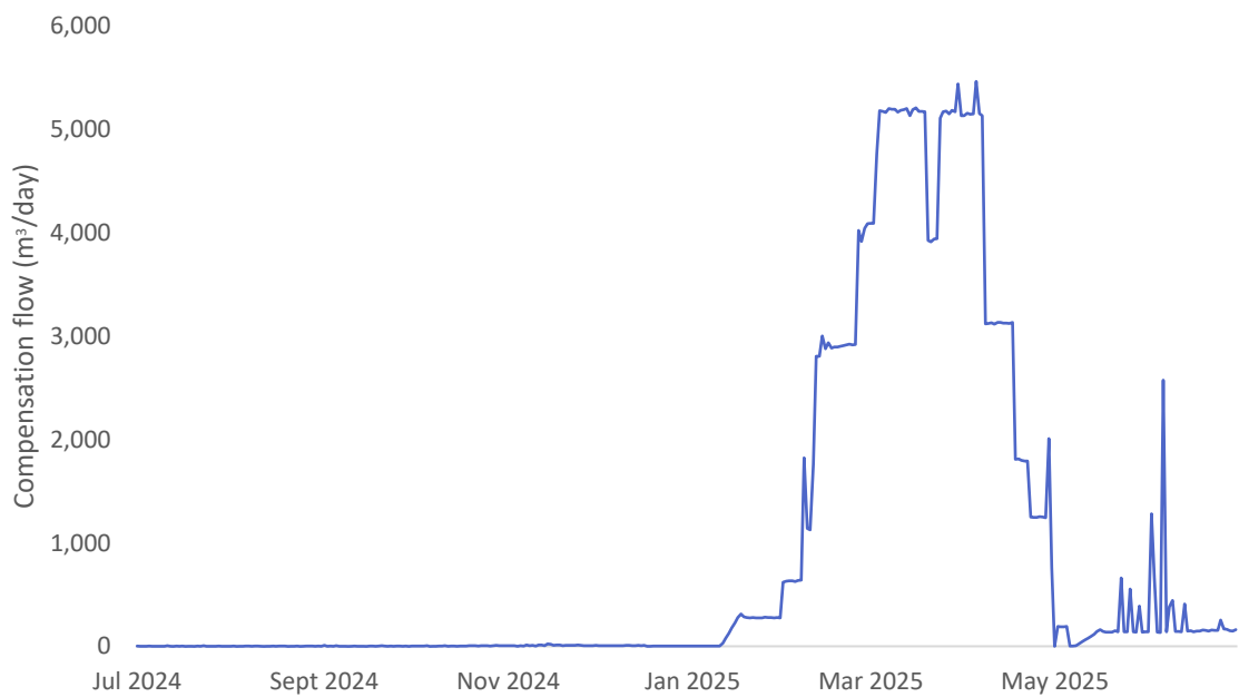
Figure 4-3: Cosseys Dam compensation flows for the reporting period 2024-2025.
