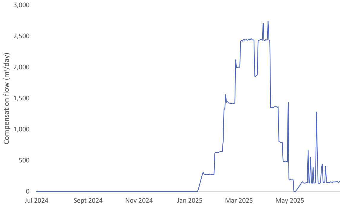
Figure 4-3: Cosseys Dam compensation flows for the reporting period 2024-2025.
